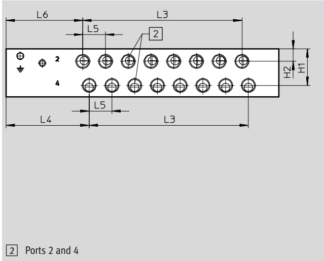
Size 14, I-Port interface, outlet on top
